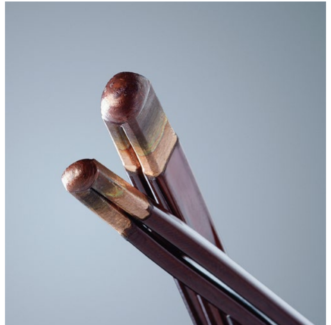
Hairpin welding for electric drives: In preparation for hairpin welding, short-pulse lasers are used to ablate the insulating varnish layer without damaging the copper underneath.
