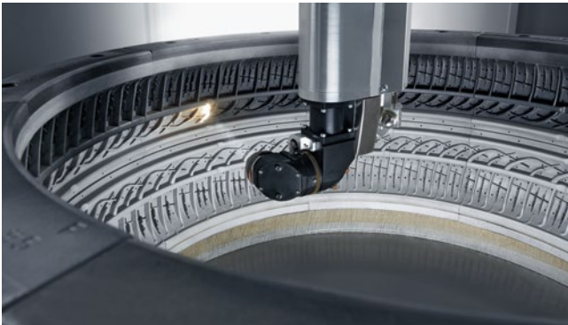
Short-pulse lasers of the TruMicro Series 7000 are the ideal tool for the efficient and profitable cleaning of tire moulds.
